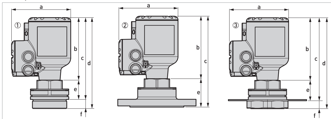
Figure 2-18: DN70 / 2 \frac{3}{4} " Lens antenna versions
